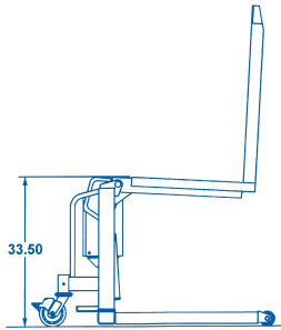
EZ Tilter® Non-straddle Models MST 20 & 40
